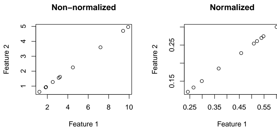
Figure 4: Non-normalized and normalized associations between feature 1 and feature 2
