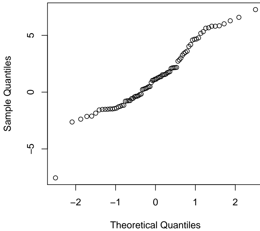
Figure 1: The per category qq-plot.
