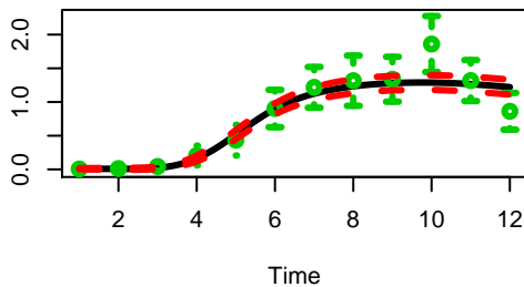
FBgn00033188 mRNA
