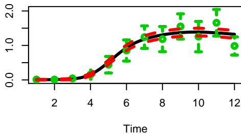
FBgn00033188 mRNA
